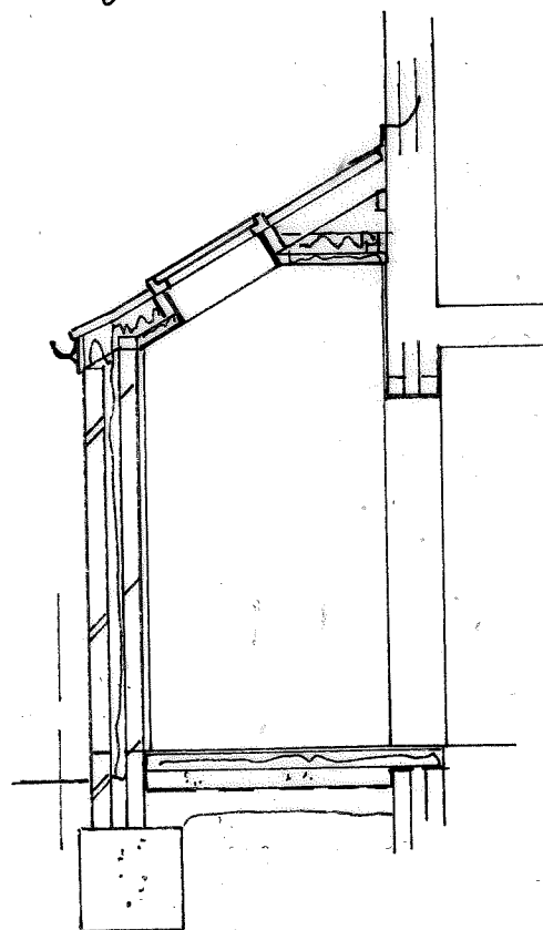
SECTION 1:50
